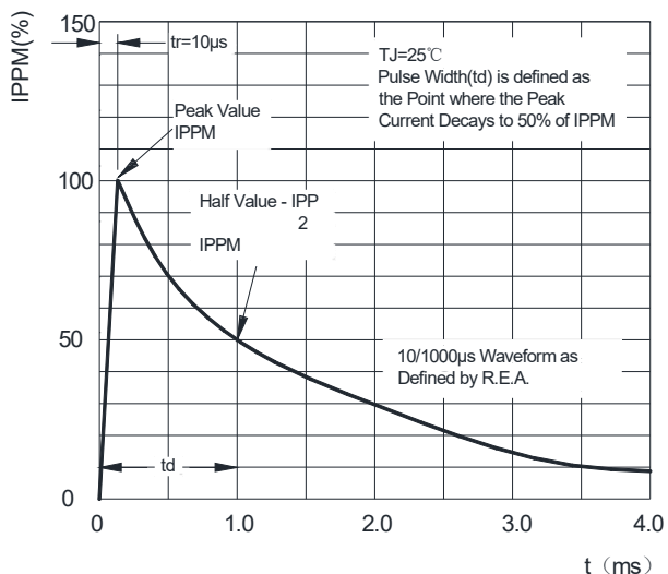
FIG3: Pulse Waveform
